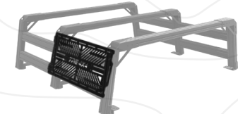
( Fixed Side Panel) TRMBR-AS-SP (742.4*382.53MM)
