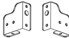
2X bracket A
